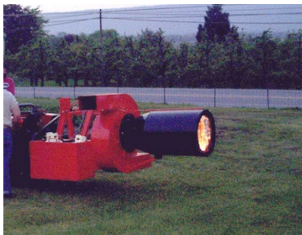
Figure 4.7 Frost Protection Using a Mobile Propane Heater (Photo by R. Crassweller).
